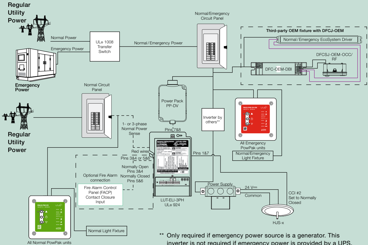
System Wiring Diagram (Vive hub with 347V emergency dimming module)
