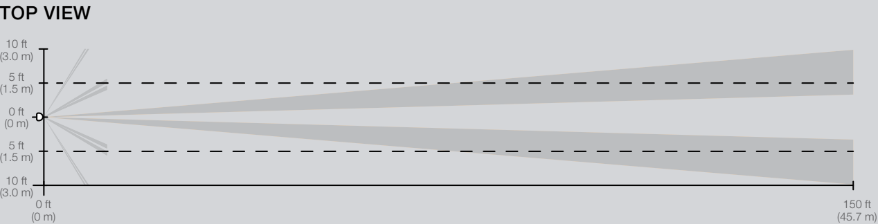
HALLWAY SENSOR MAXIMUM RECOMMENDED LENGTH CHART (sensor centered within hallway)
