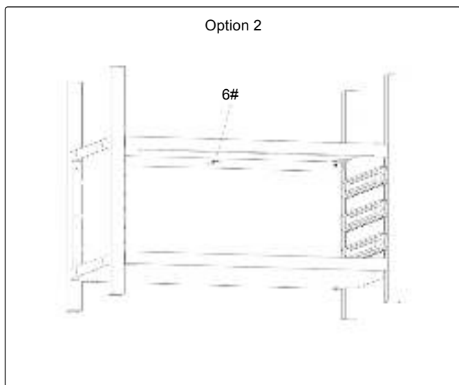
Step 7. Fix the cabinet to the wooden wall with the self-tapping screw ST4.8*30, no wall plug is required.
