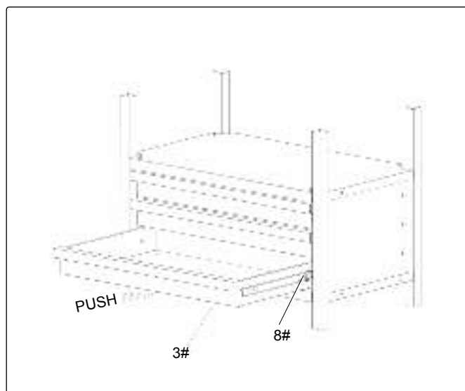
Step 8. Assembly of the drawers. For easy drawer removal, release levers on both sides of drawer as shown in the diagram.
