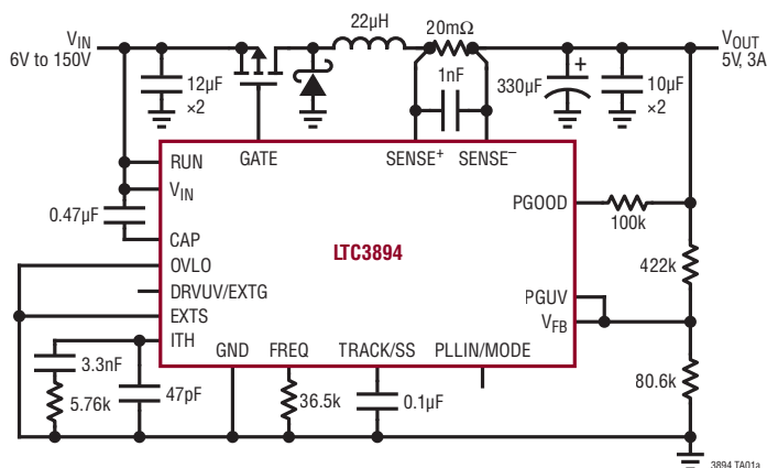
High Efficiency 150V to 5V Step-Down Regulator
