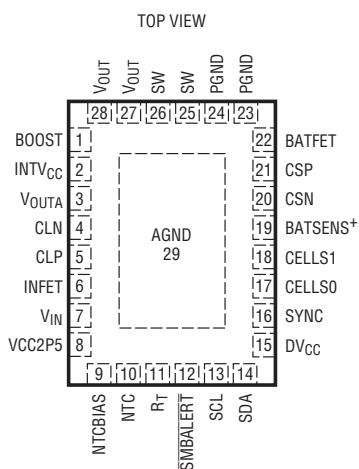
UFD PACKAGE 28-LEAD (4mm × 5mm) PLASTIC QFN
