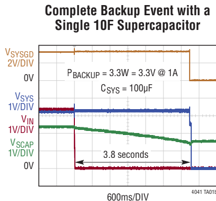
Single Supercapacitor 3.3V Backup Application
