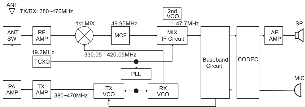
Fig.1 Frequency configuration
