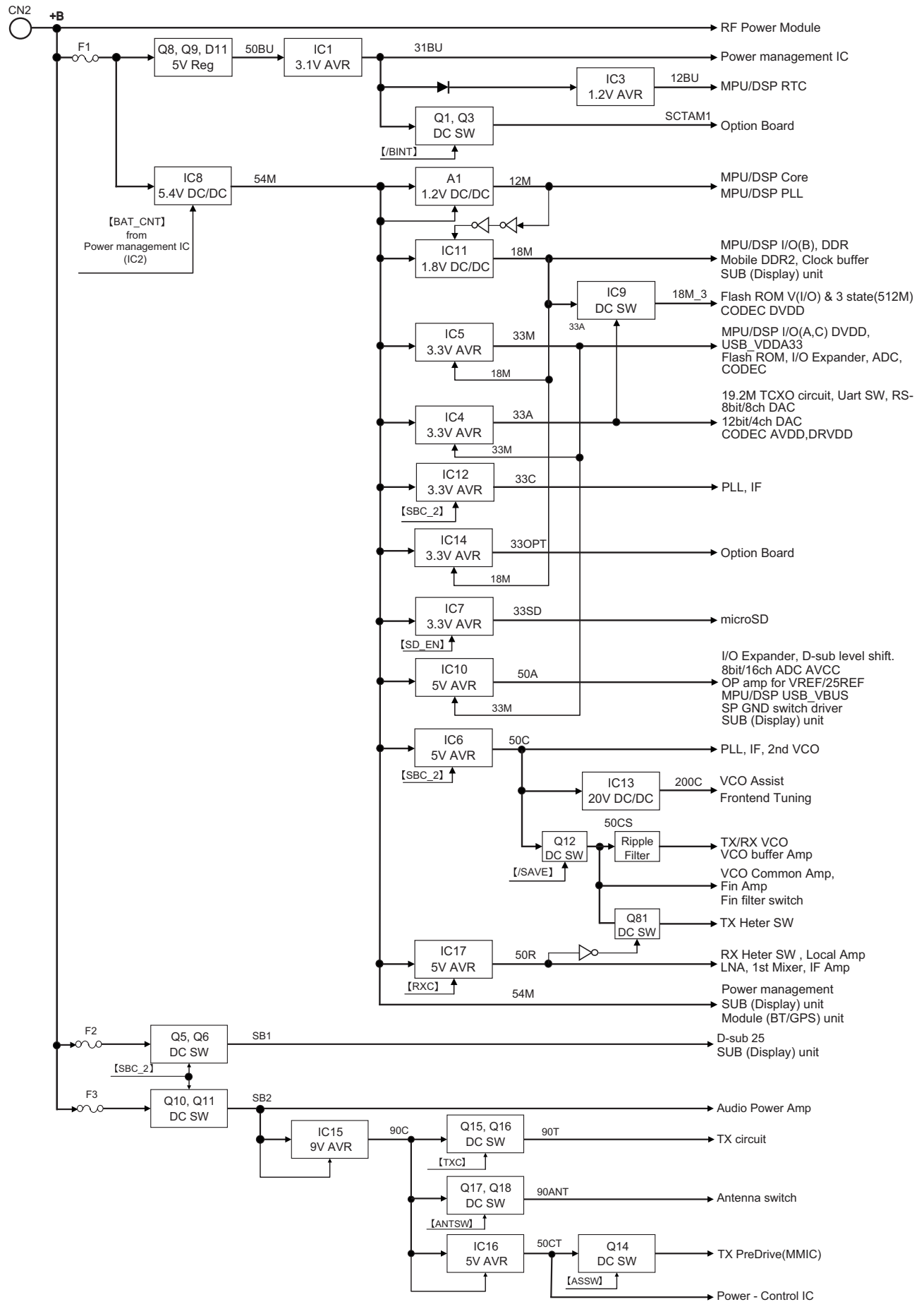
Fig.4 Power supply circuit
