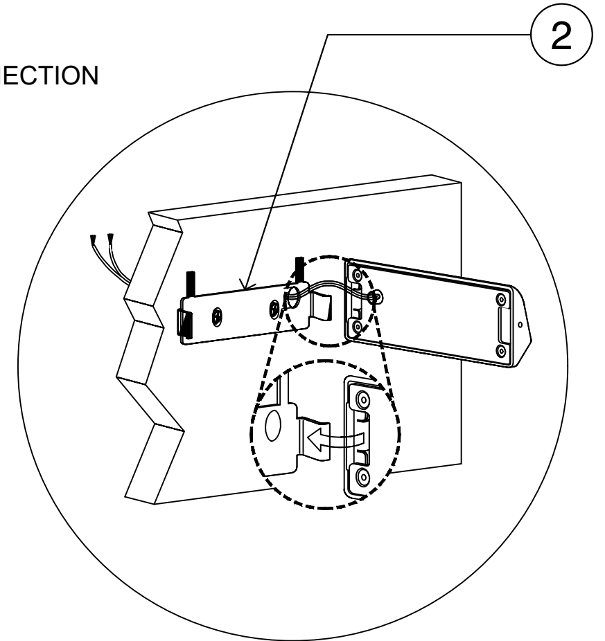
MOUNTING DETAIL
