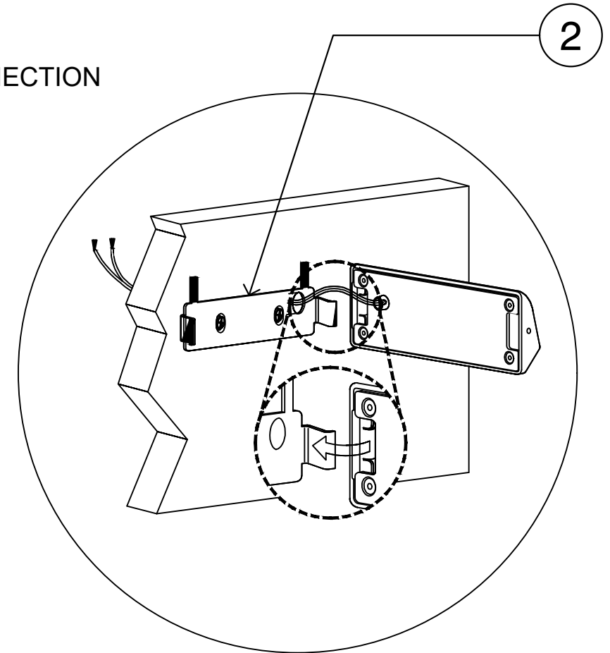
MOUNTING DETAIL
