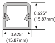
INF-X-CHAN-8 X = C (clear), F (frosted) Polycarbonate extrusion available in 8' length
