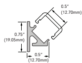
TPL-I-45-MCH-8 White PVC 45° extrusion INF-X-LNS-8 X = C (clear), F (frosted) Polycarbonate lense available in 8' length
