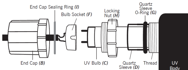
Figure 4. Quartz Sleeve
