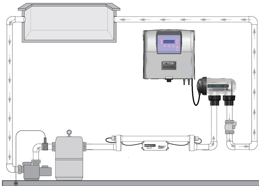
Figure 3. Installation Position
