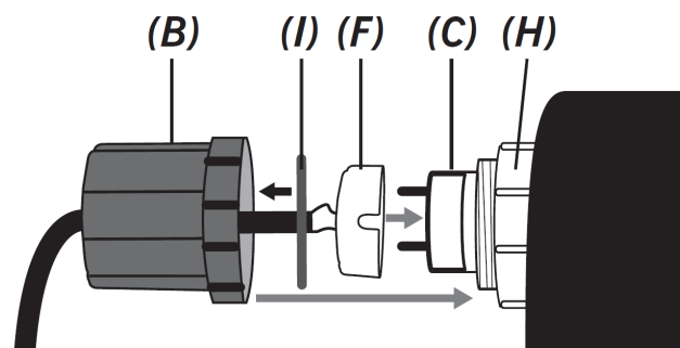
Figure 5. UV Bulb
