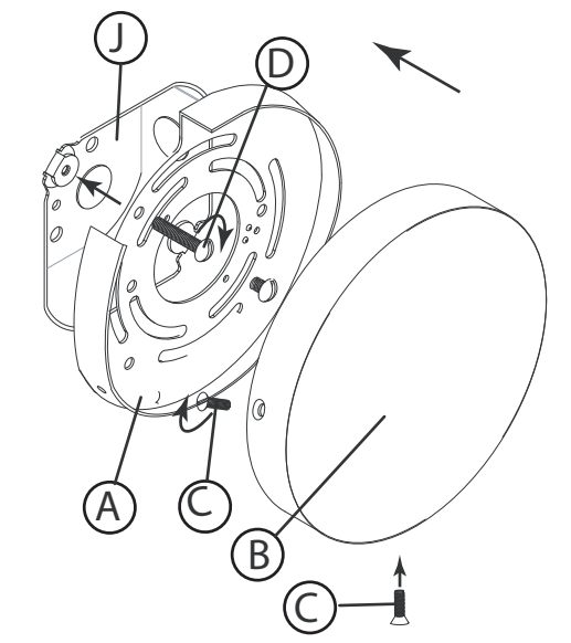
DRAWING 2 - Mounting without Jbox
