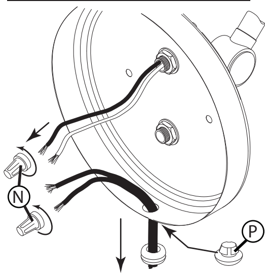
DRAWING 3- Removing plug
