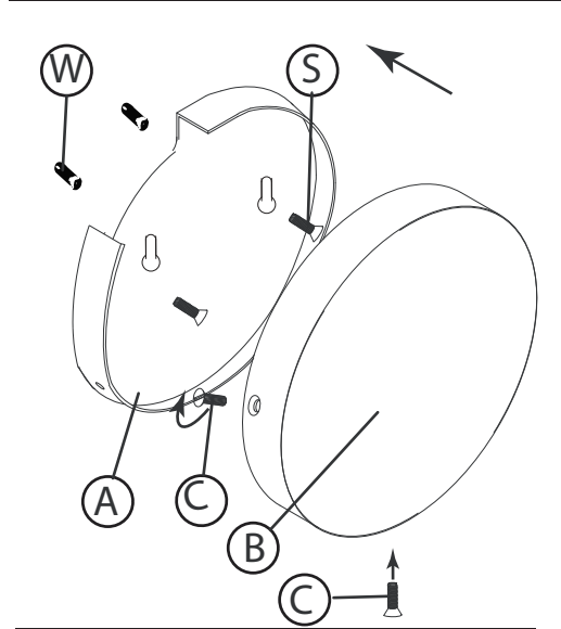
DRAWING 3- Removing plug
