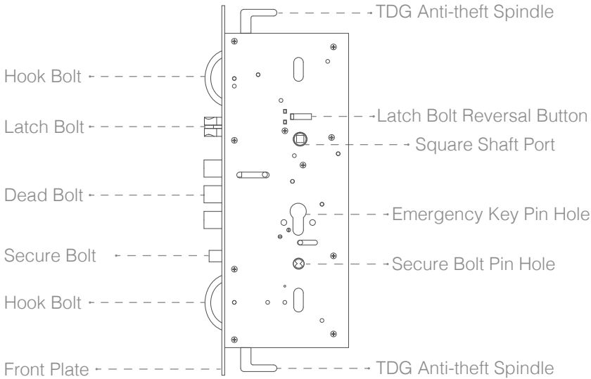
388 Lock Body (Optional)
