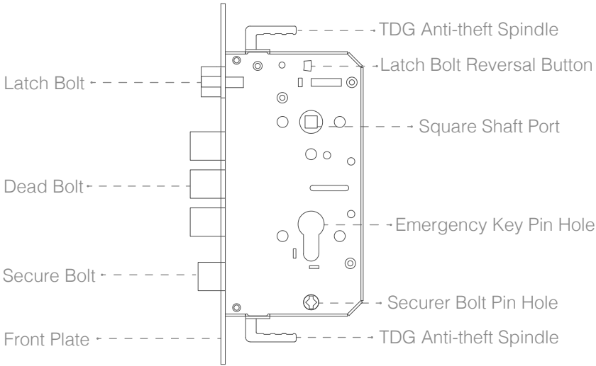
30 * 240 Lock Body (Optional)
