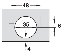
Hinge Drilling Pattern
