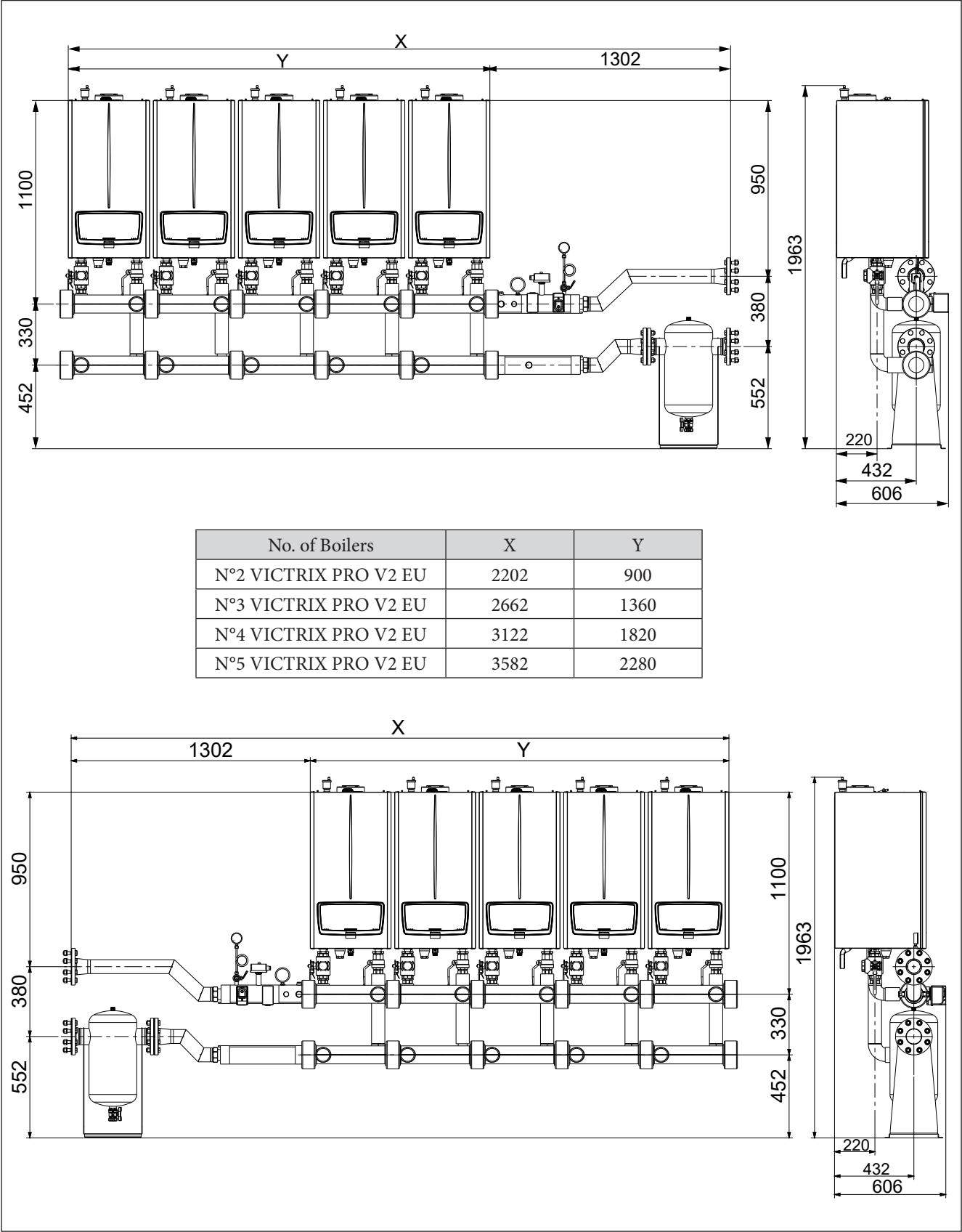
21.3 DIMENSIONS AND CONNECTIONS WITH RH/LH SLUDGE REMOVER KIT FOR VICTRIX PRO V2 35 - 55 - 60 - 68 - 80 EU IN SET INSTALLATION (CODE: 3.033674) (UP TO A MAXIMUM OF FIVE APPLIANCES)
