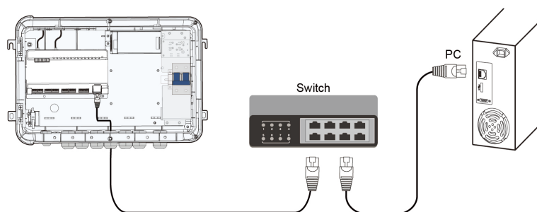
figure 4-2 Connecting to Background of PV System
