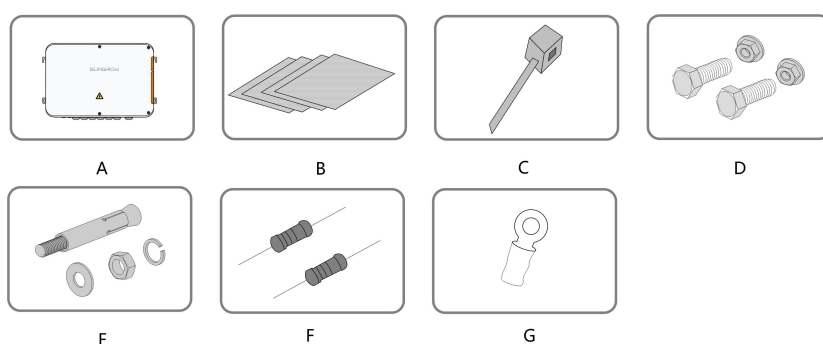
figure 3-1 Packing List
