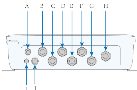
figure 4-1 Waterproof Terminals on Bottom of COM100
