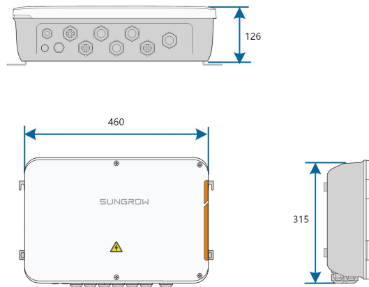
figure 2-2 Dimensions of COM100 (mm)
