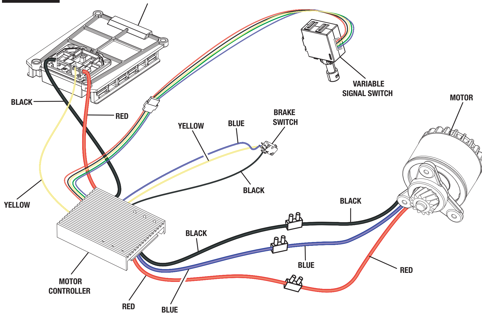
WIRING DIAGRAM
