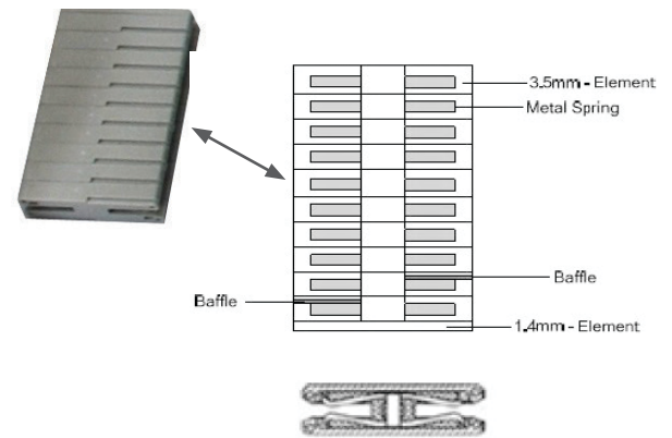
Figure 5: Board-to-Board Connector
