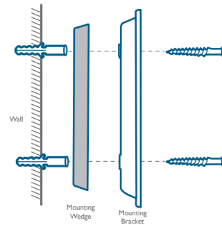
With 15^\circ Mounting Wedge
