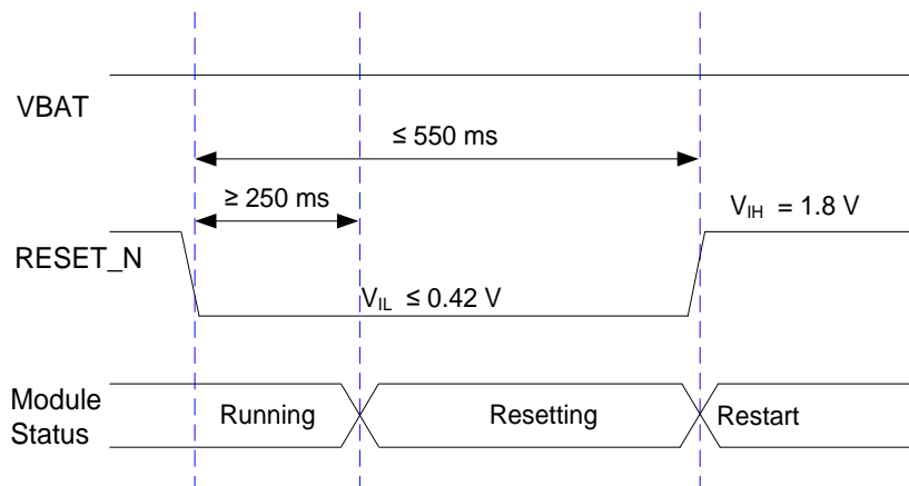
Figure 15: Reset Timing
