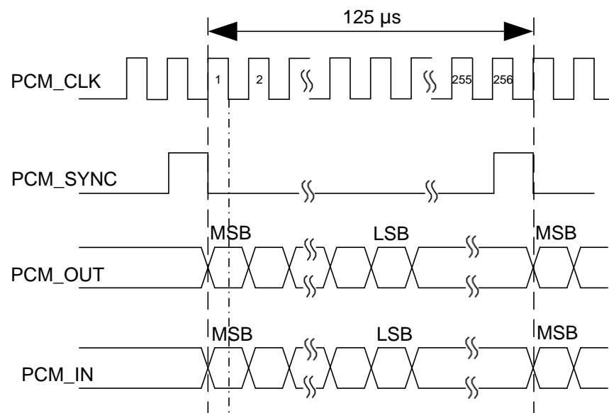
Figure 22: Short Frame Sync Mode Timing
