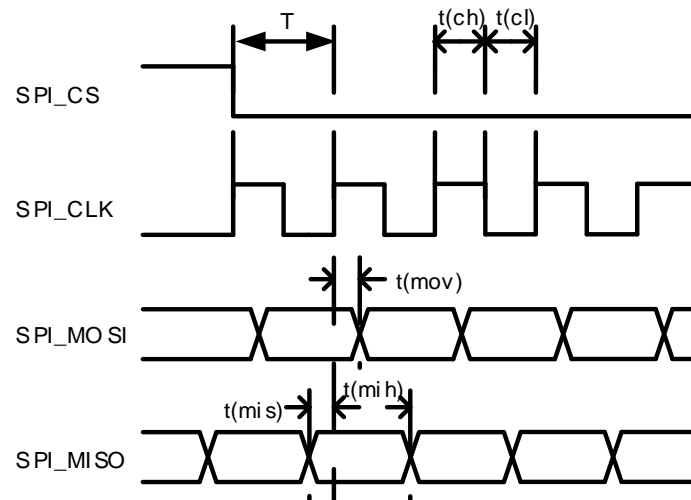
Figure 25: SPI Timing
