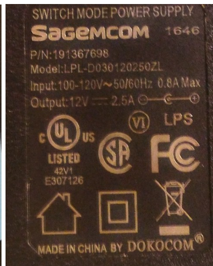
POWER SUPPLY
