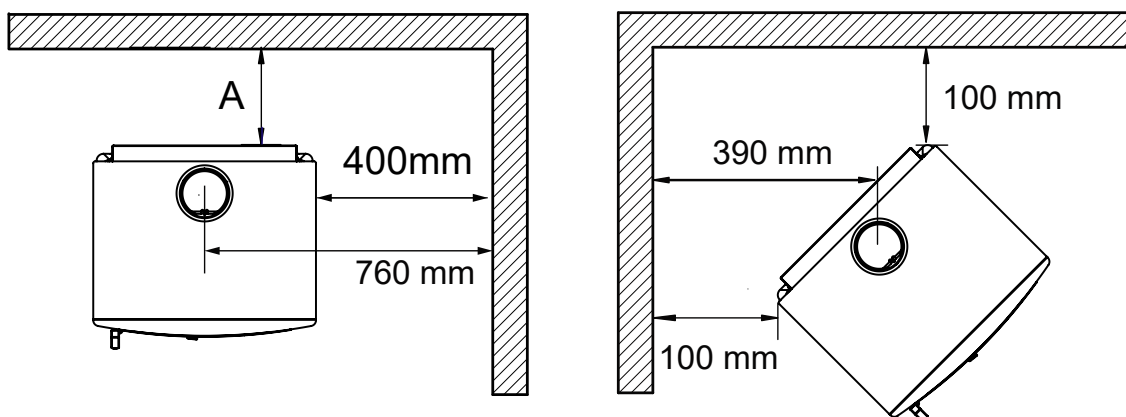
Figure 5. AB25 AUS CLEARANCES.
