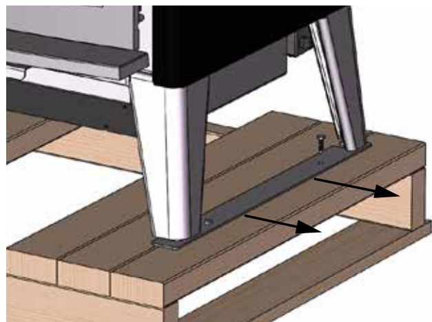
Figure 2. AB25 Hold down removal1.
