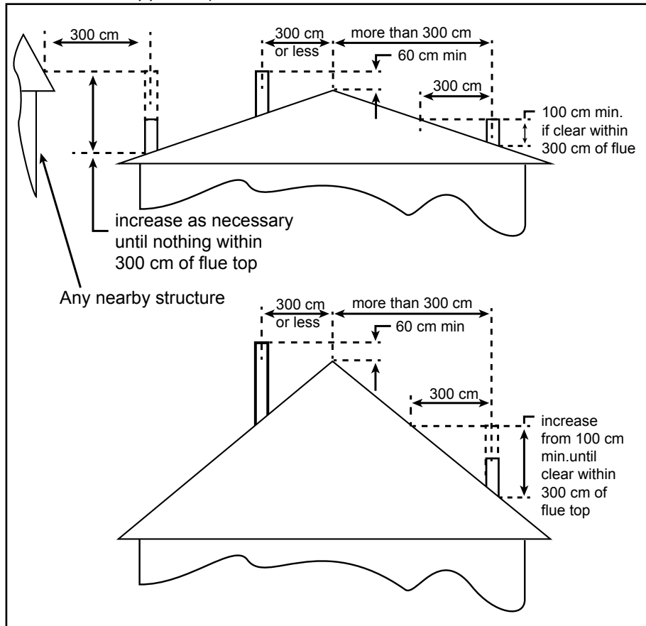
Figure 7. Neo 1.6 Chimney and connector
