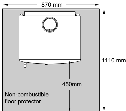
Figure 6. AB25 AUS Floor protection.
