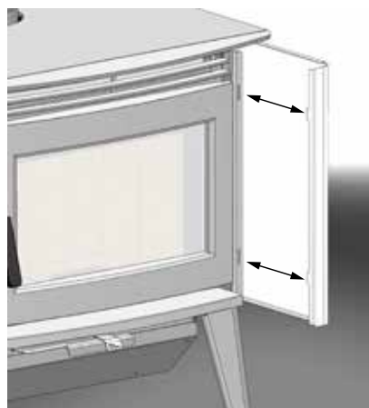
Figure 4. AB25.Side panel tab install.
