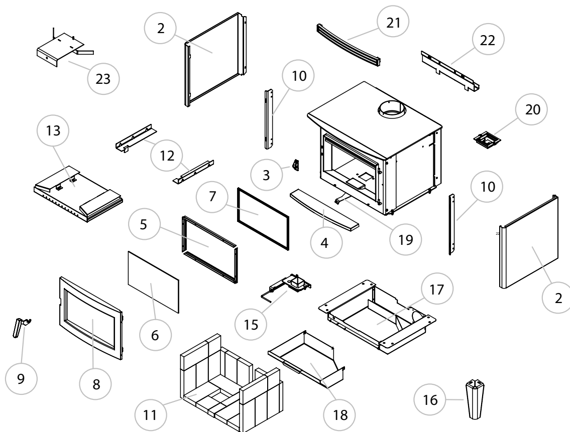
Figure 10. AB25.Exploded Parts.
