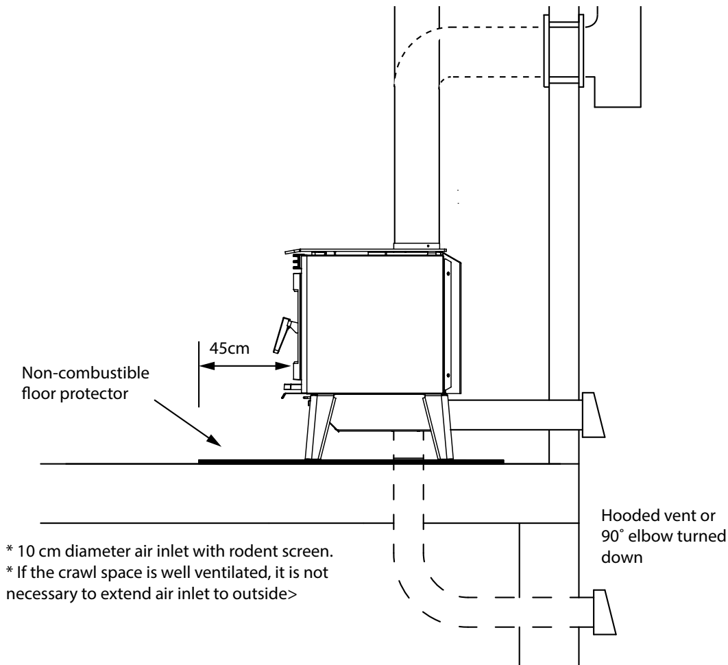
Figure 9. AB25 AUS INSTALL Diagram.
