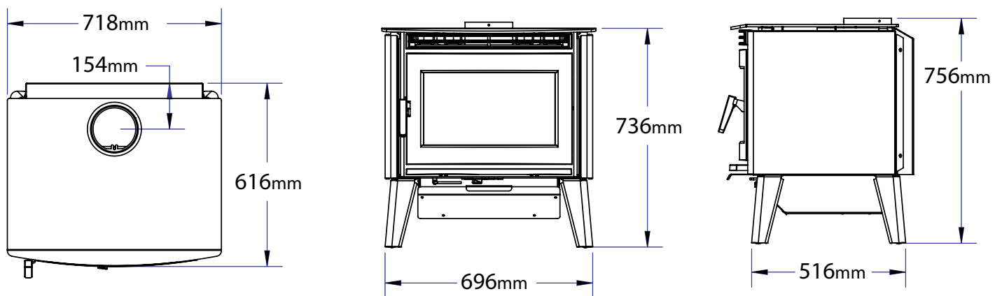
Figure 1. AB25 Dims metric.
