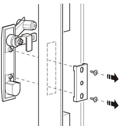
Typical door
