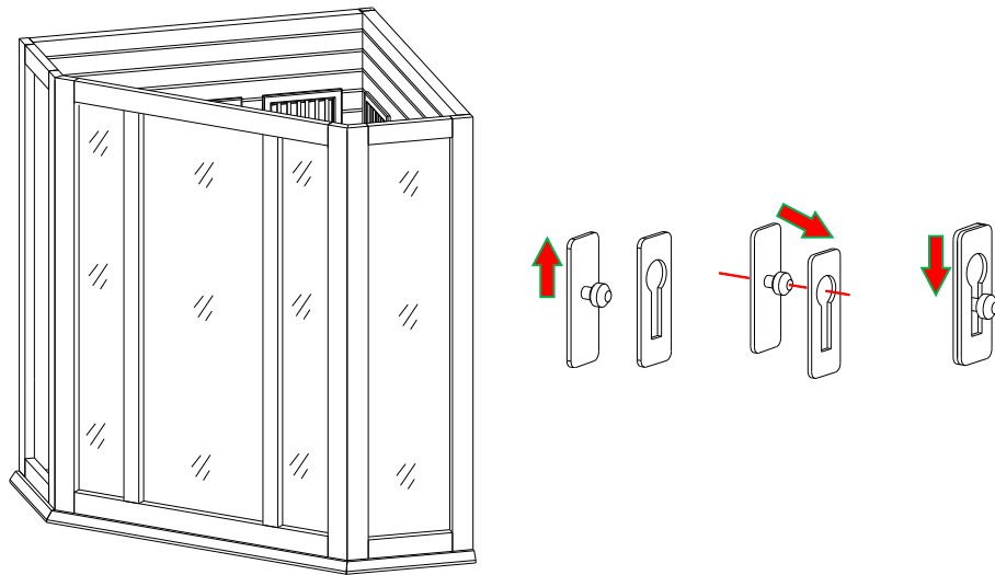
FIG-11 Assembling Front Panel
