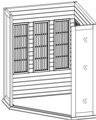
FIG-6 Assembling Back Side Panels and Side Panels
