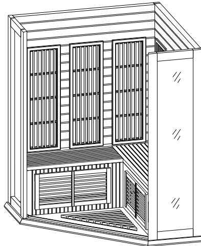
FIG-9 Inserting Benches screws
