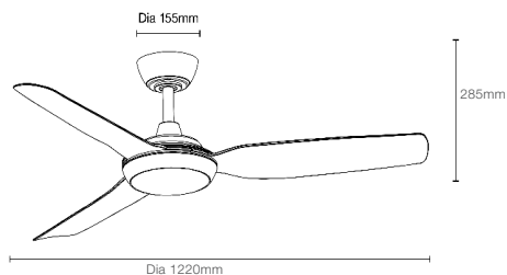
1220mm (48") Model
