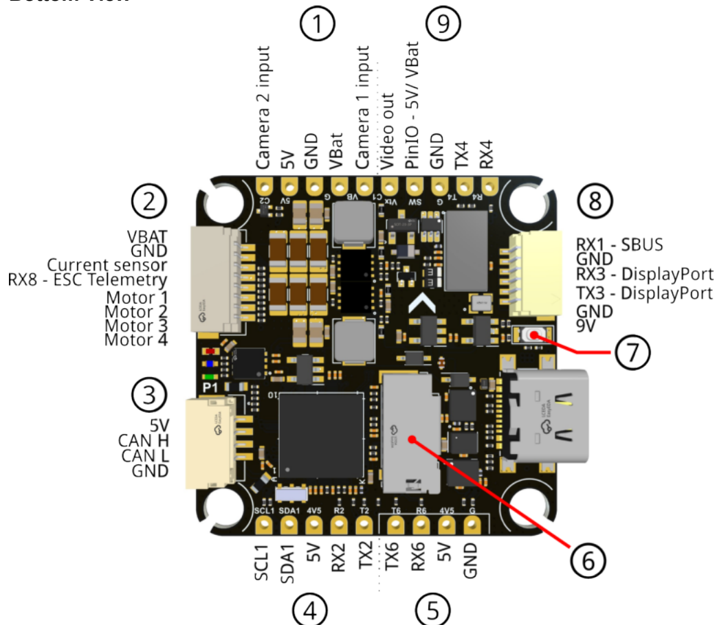
Bottom View
