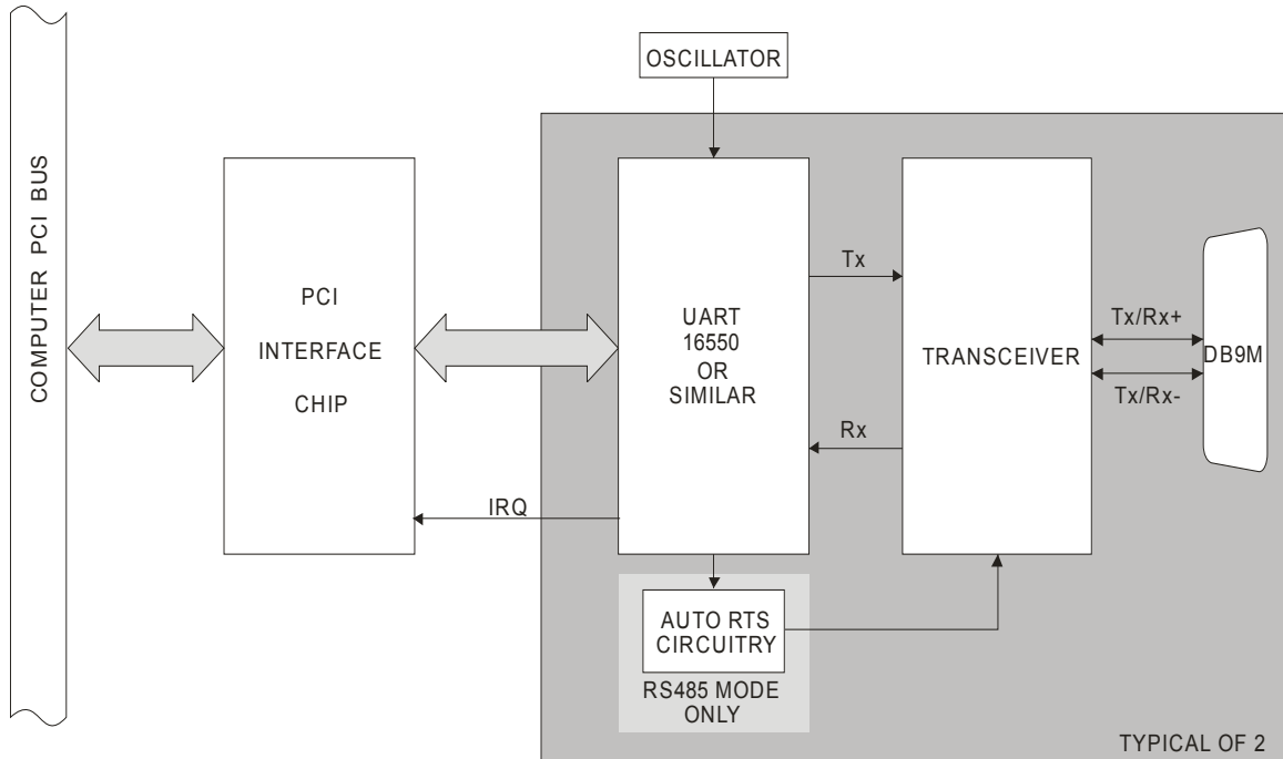
Figure 1-1: Block Diagram
