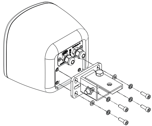
Figure 5.10: Mounting plate
