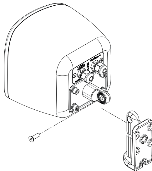
Figure 5.5: Wall mounting
