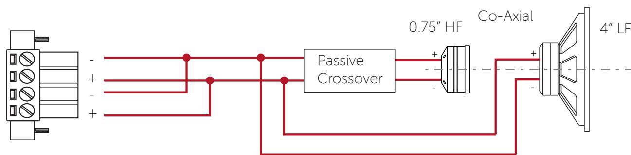
Figure 4.2: Wiring diagram
