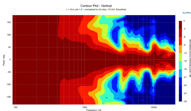
Figure 3.2: Vertical directivity isobars
