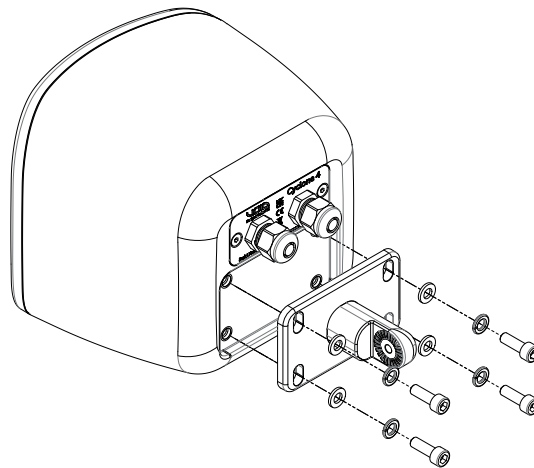
Figure 5.4: Attach plate
