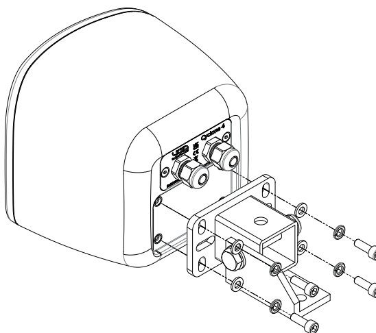
Figure 5.14: Stud bracket attachment
