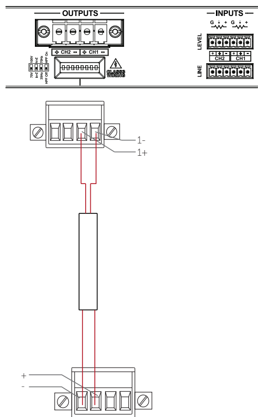
Figure 4.3: Bias D1
