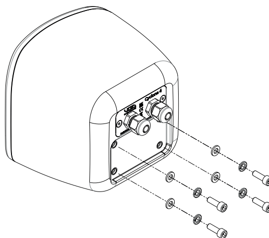
Figure 5.8: Mounting plate removal
