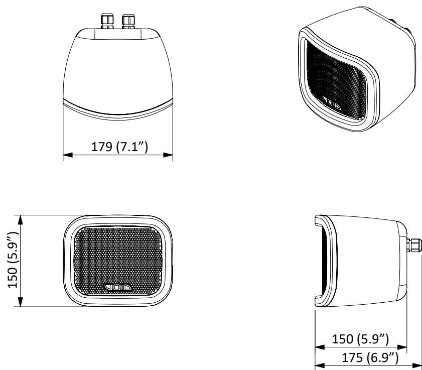
Figure 3.3: Dimensions
