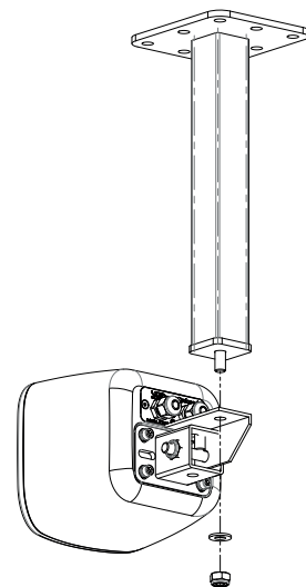
Figure 5.11: Ceiling mounting
