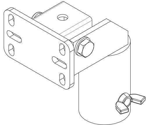
Figure 5.15: T51 pole bracket kit
