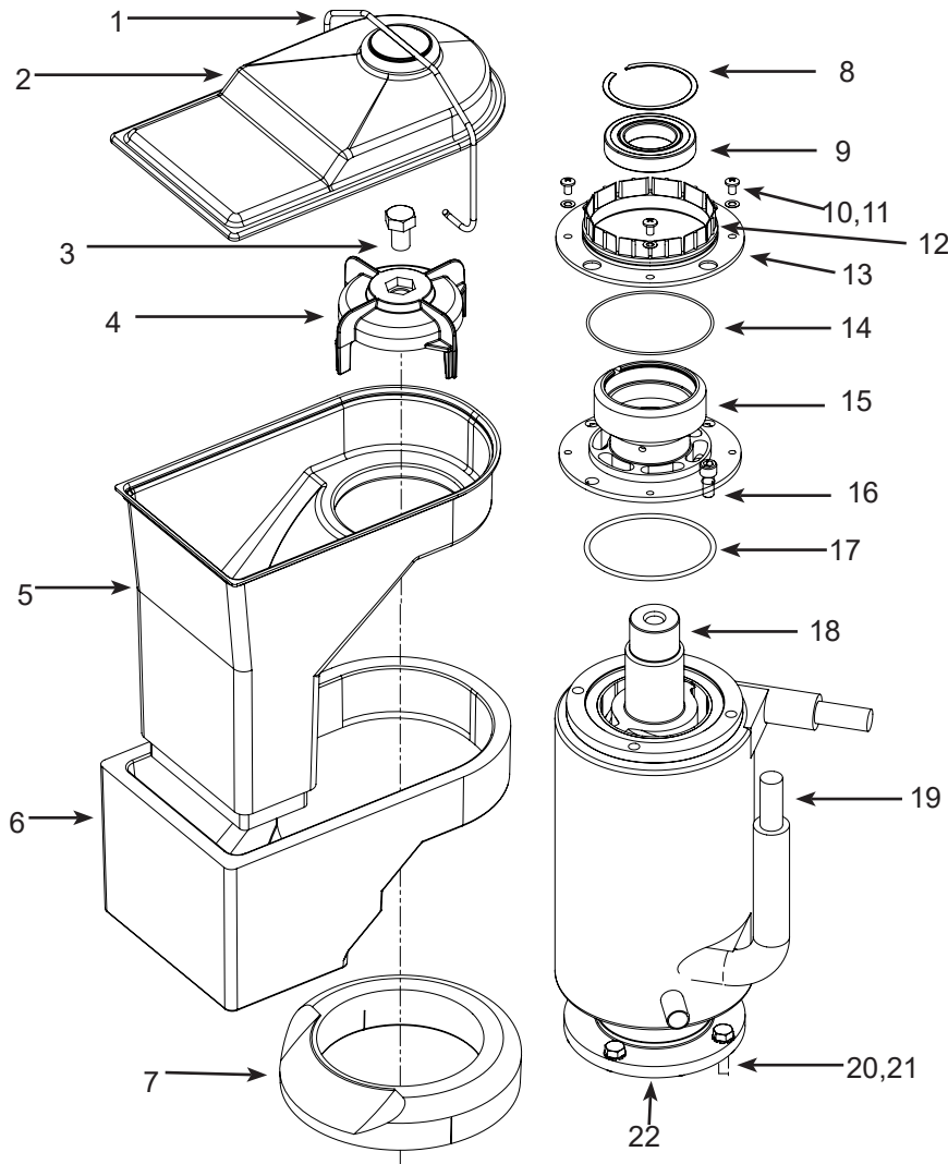
Flaker
