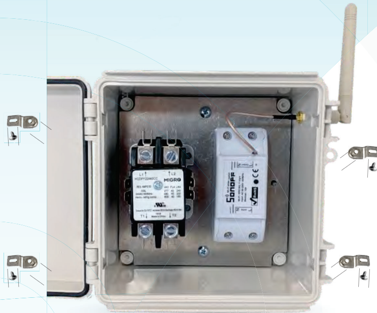
IMAGE 1. Mounting Brackets
