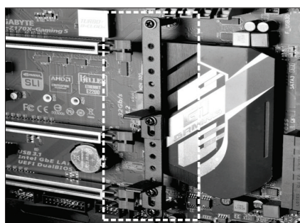
GB-001X Graphic card anti-sag bracket
