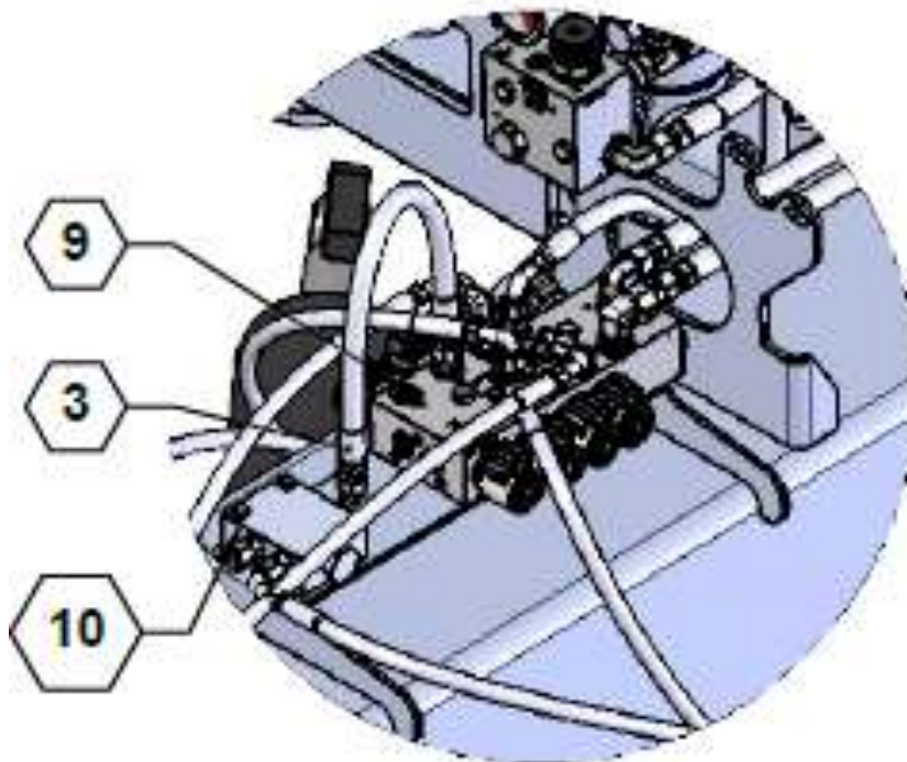
DETAIL E
