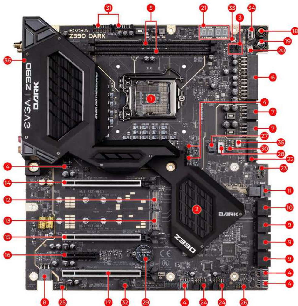
FIGURE 1. Z390 DARK Motherboard Layout
