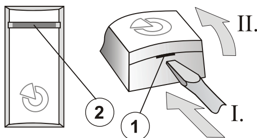
Figure: 1 – cover tab; 2 – red activation indicator
