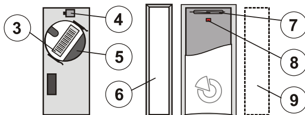
Figure: 3 – production code; 4 – tamper contact; 5 – battery; 6 – permanent magnet; 7 – magnetic sensor; 8 – red detector activation indicator; 9 – alternative location of the permanent magnet
