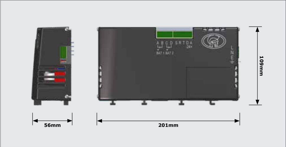
FIGURE 1. SMART POWERPACK PHYSICAL DIMENSIONS
