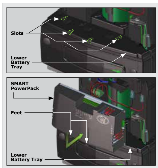
FIGURE 8. SMART POWERPACK PLACEMENT
