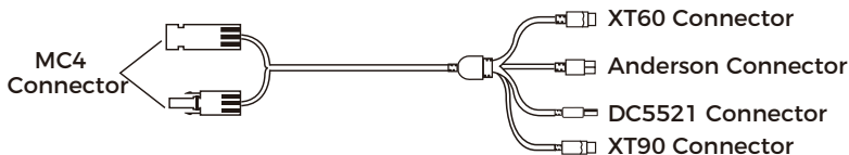
MC4 to XT60/XT90/Anderson/DC5521 Adapter Cable
