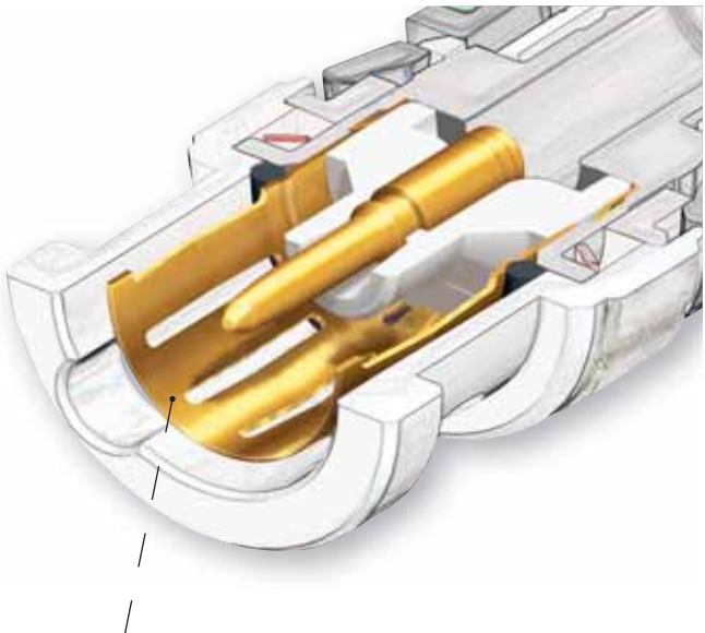
Gold plated ground contact with improved shielding effectiveness optimized for high frequency HDTV signal up to 3 GHz.
