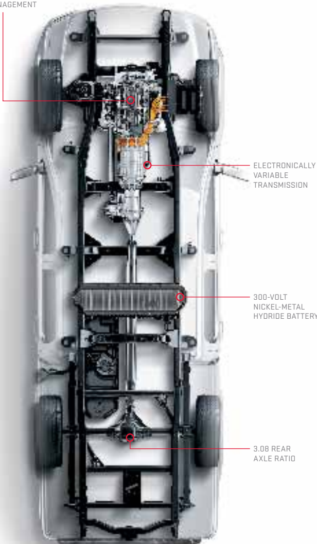
SIERRA HYBRID CHASSIS AND POWERTRAIN
