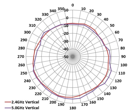
E-Plane Pattern
