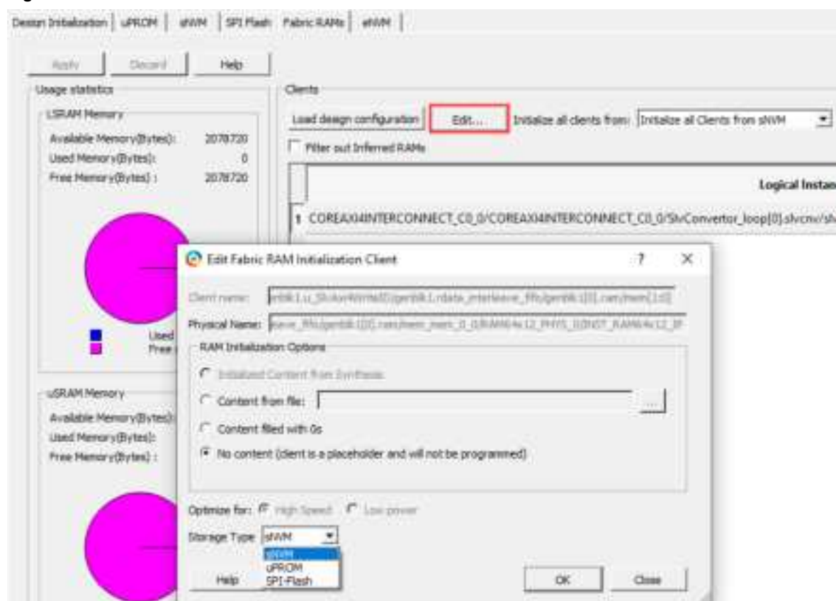
Figure 2-10. Fabric RAMs
