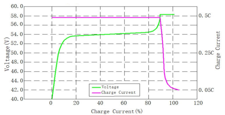
Charging Characteristics @0.5C 25°C
