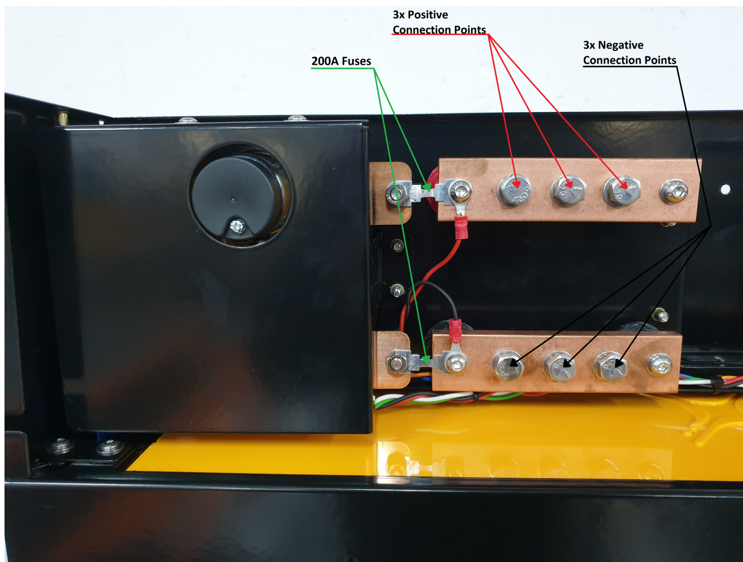
Figure 5 connection terminals
