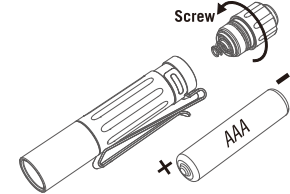
AAA Alkaline Battery ( Installed Inside the Flashlight )
