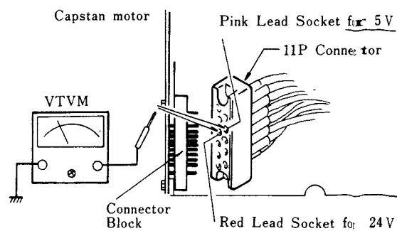
Fig. 8-4 Test Points
