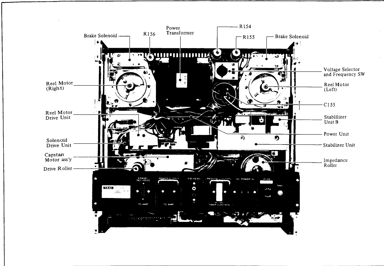
Fig. 5-1 — Mechanical Section —
