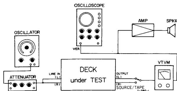
Fig. 10-8 Test Connections for Monitor Check
