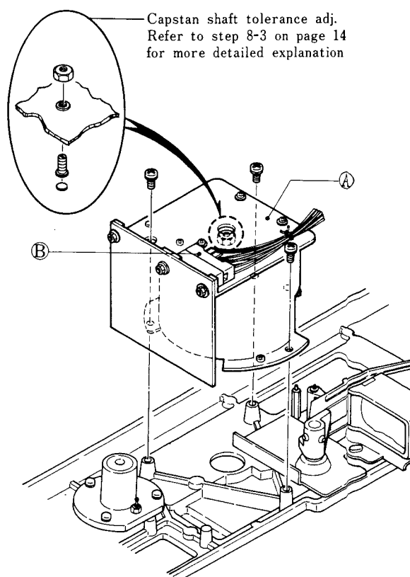
Fig. 4-8 Capstan Motor ass'y Removal
