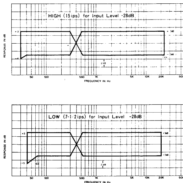
Fig. 10-15 Frequency Response –OVERALL– 3
