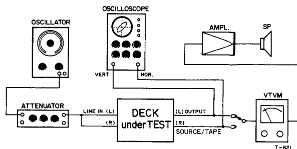
Fig. 10-11 Test Connections for Recording Check
