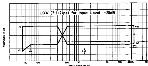
Fig. 10-13 Frequency Response —OVERALL — 1
