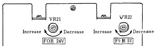
Fig. 8-3 Adjustment Location
