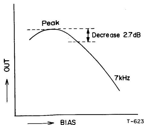
Fig. 10-12 Bias Limits Chart
