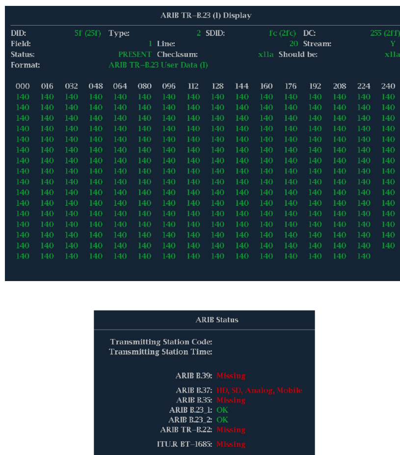
Figure 69: ARIB TR-B.23 (1) display (with the associated ARIB Status display)
