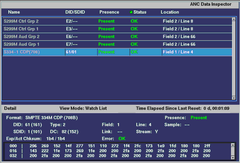
Figure 10: ANC Data display (full screen mode)
