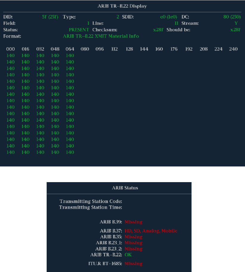
Figure 71: ARIB TR-B.22 display (with the associated ARIB Status display)
