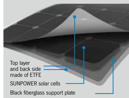
Structure of the Power Panel SFX135
