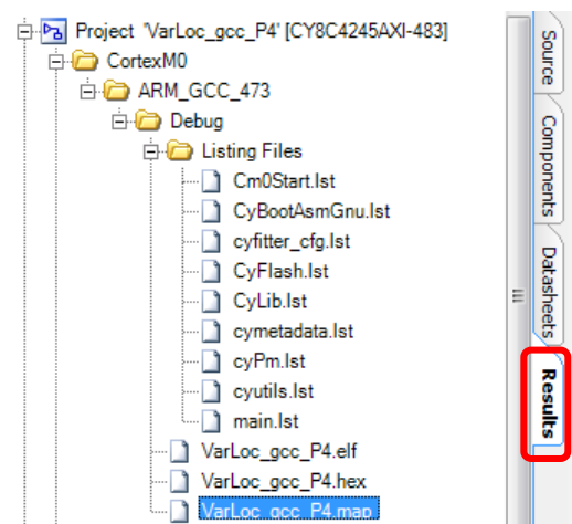
Figure 12. .map File in PSoC Creator
