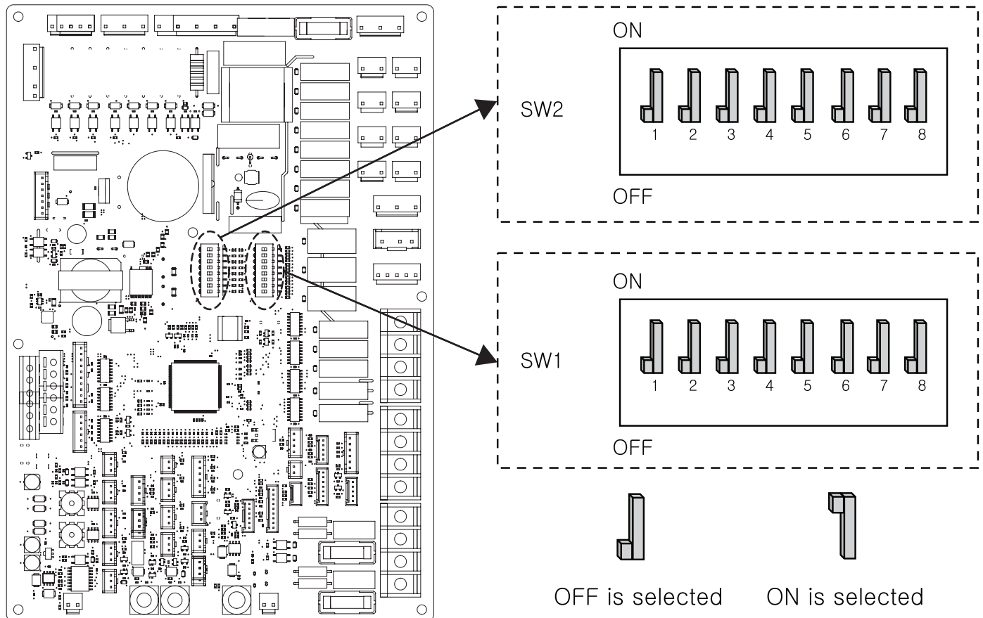
Figure 9: Dip Switch Settings.
