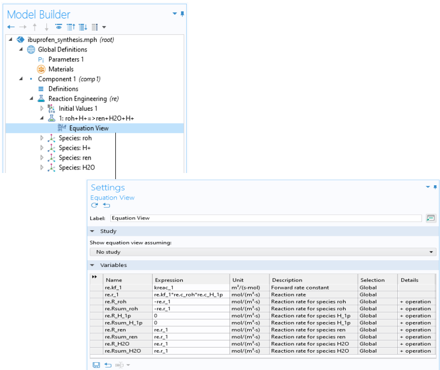
Figure 2-4: The definition of variables used by a node are accessible through the Equation View.
