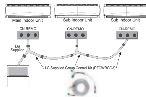
Figure 49: Example of Indoor Unit Group to Zone Controller Connections (CN-REMO).
