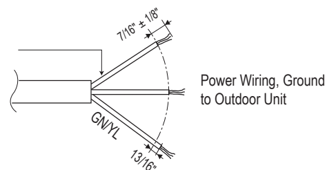
Figure 35: Multi F / Multi F MAX with LGRED Outdoor Unit Power Wiring.
