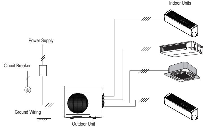
Figure 38: Typical Multi F with LGRED System General Power / Communications System Schematic When Wiring is Less Than 130 Feet.
