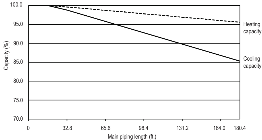
Figure 3: Multi F MAX with LGRED Outdoor Unit to Branch Distribution Unit Refrigerant Line Length Derate Chart.
