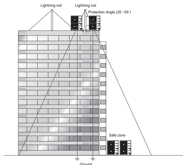
Figure 47: Lightning Protection Diagram.
