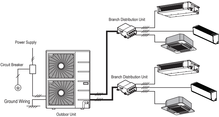
Figure 39: Typical Multi F MAX with LGRED System General Power / Communications System Schematic When Wiring is Less Than 130 Feet.
