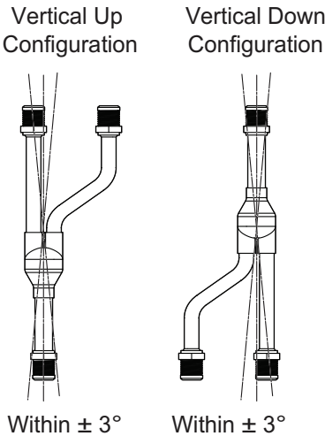
Figure 31: Y-branch Installation Alignment Specification.
