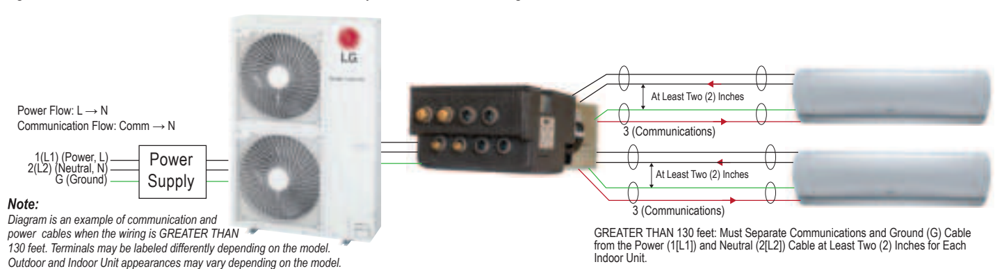
Figure 41: Schematic of a Multi F MAX with LGRED System When the Wiring is GREATER THAN 130 Feet.
