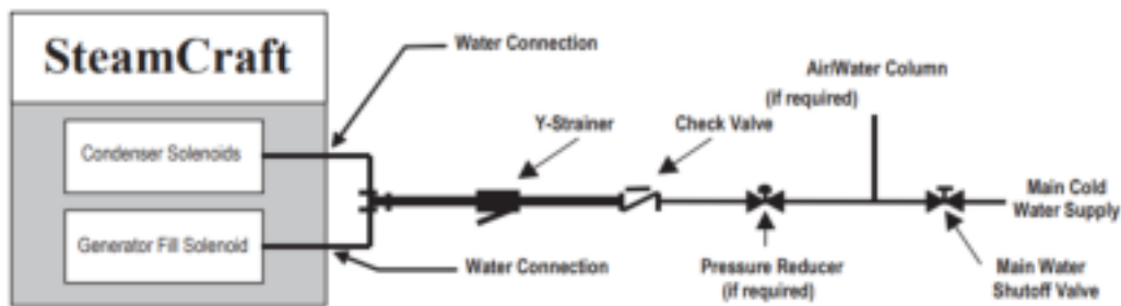
Figure 3-2 Cleveland Range Single Water Supply Arrangement
