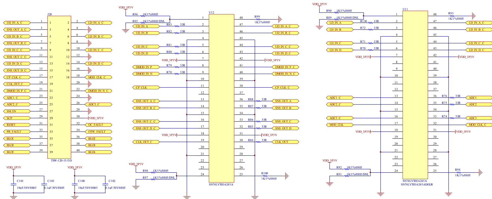
Figure 25. Line Drivers and Dual Row Header
