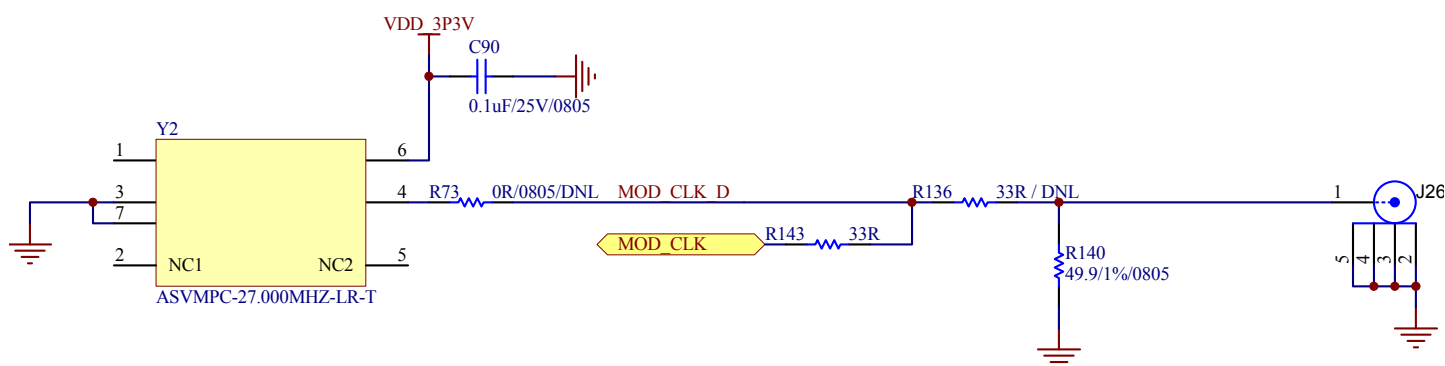
Figure 14. MOD_CLK Internal 27MHz Oscillator and External SMA Input Schematic
