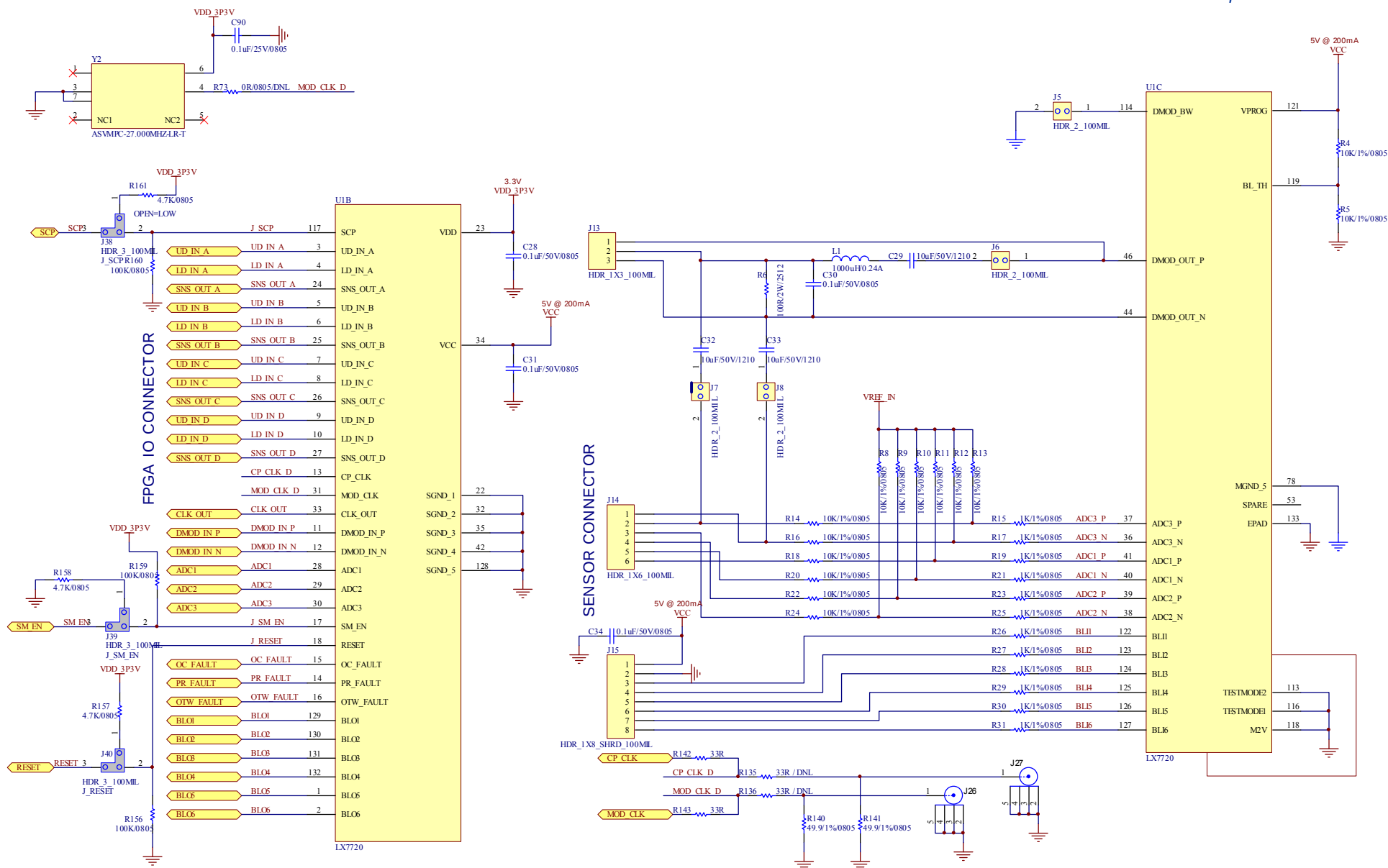
Figure 23. FPGA and Sensor Connection
