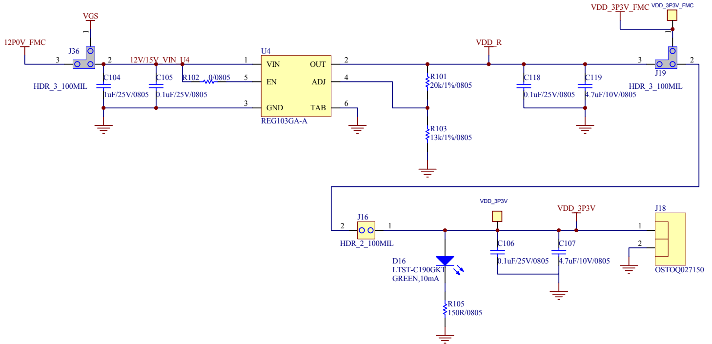
Figure 10. VDD Logic Supply (3.3V) Regulator Schematic
