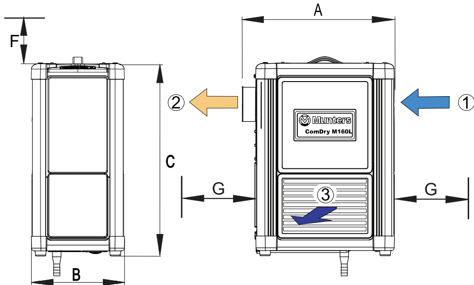
Figure 10.1 Dimensions, ComDry M160L
