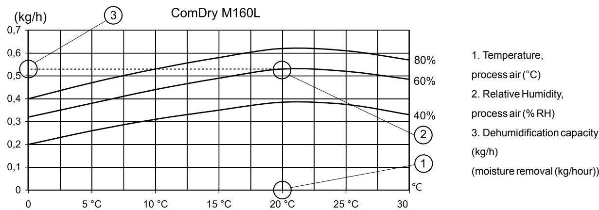
Figure 10.2 Capacity diagram
