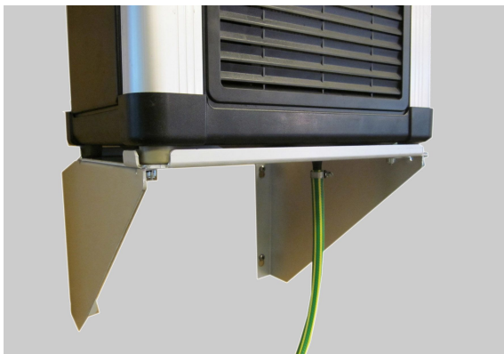
Figure 4.5 Drain hose connection
