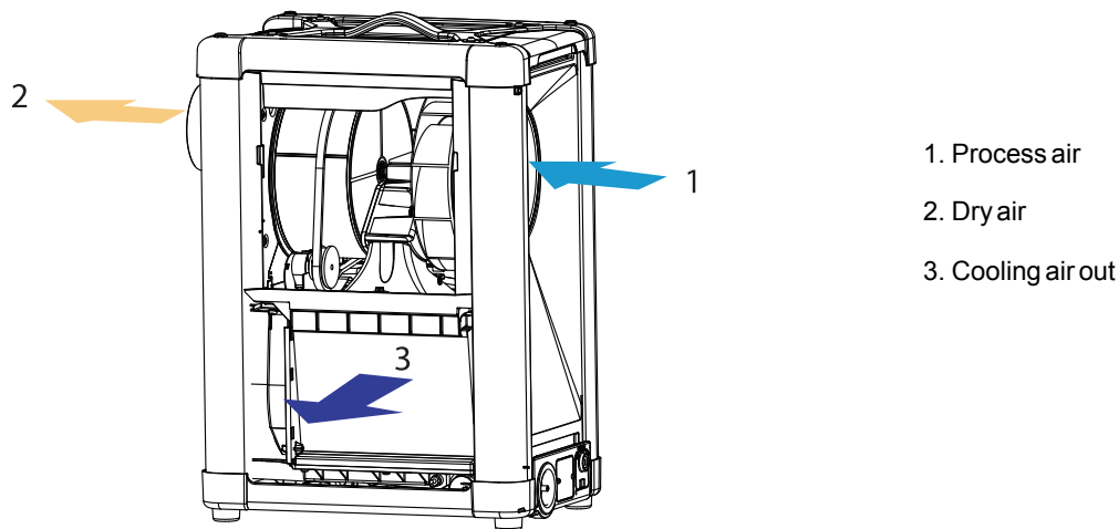
Figure 2.1 Principle of operation
